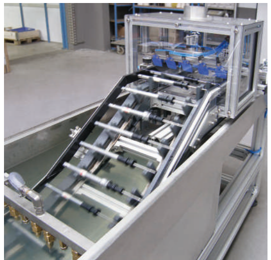
TKU 2040 with 20° inclination and transport of workpieces through a cleansing bath
