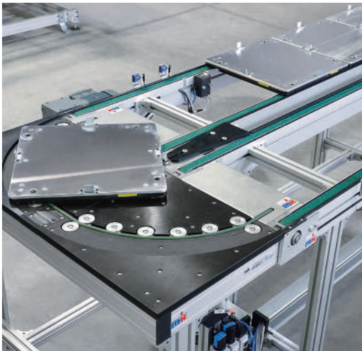
Versamove standard pallet circulation system with compact 180° KER 320 curved section
