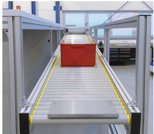
RBS-P 2255 with plastic rollers with \varnothing 40 mm
